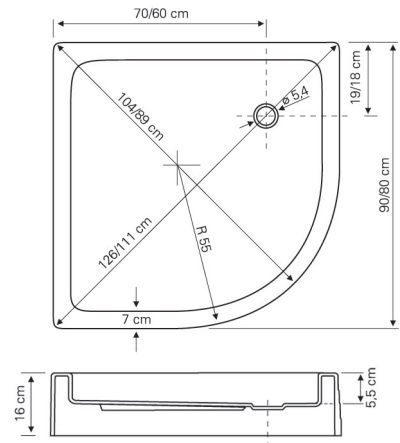
Shower tray - Tuš kada
