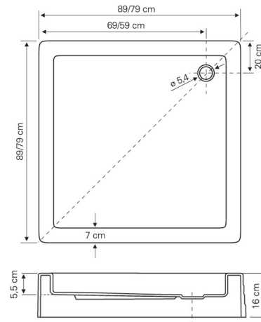
Shower tray - Tuš kada
